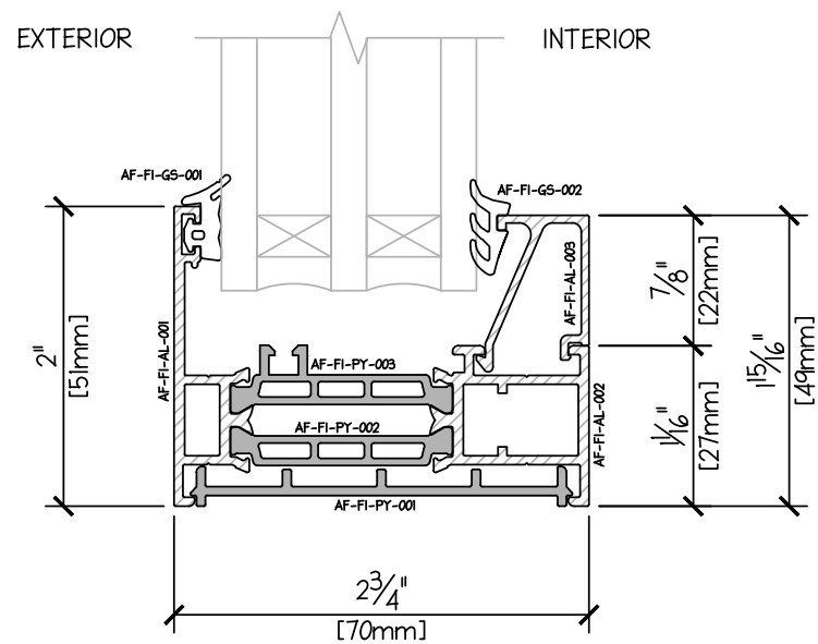
TT-FIXED PROFILE - SILL TRIPLE GLAZE 43mm
