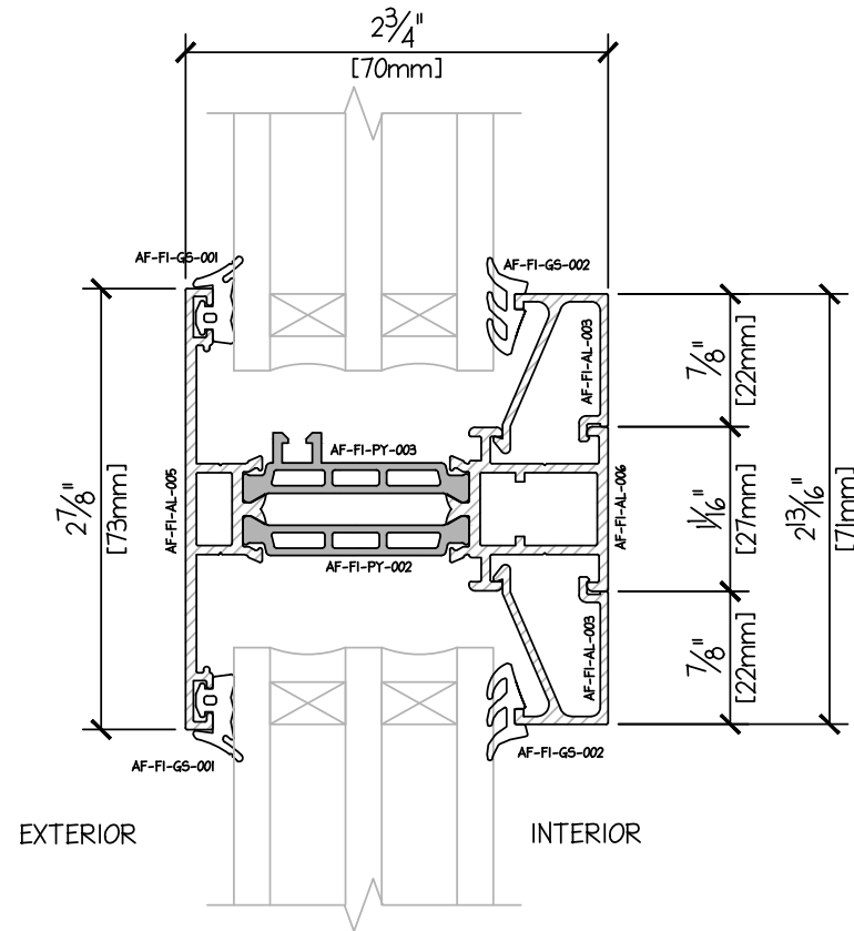
TT-FIXED PROFILE - HORIZONTAL MULLION TRIPLE GLAZE 43mm
