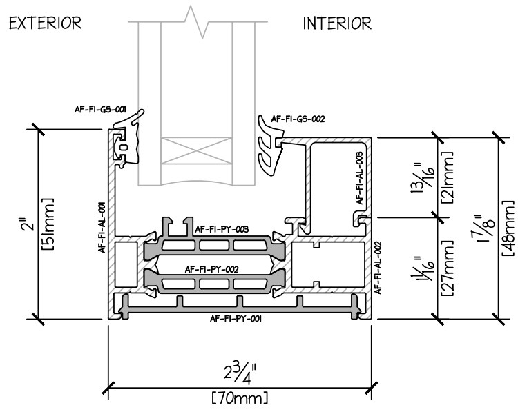
TT-FIXED PROFILE - SILL DUAL GLAZE 31mm
