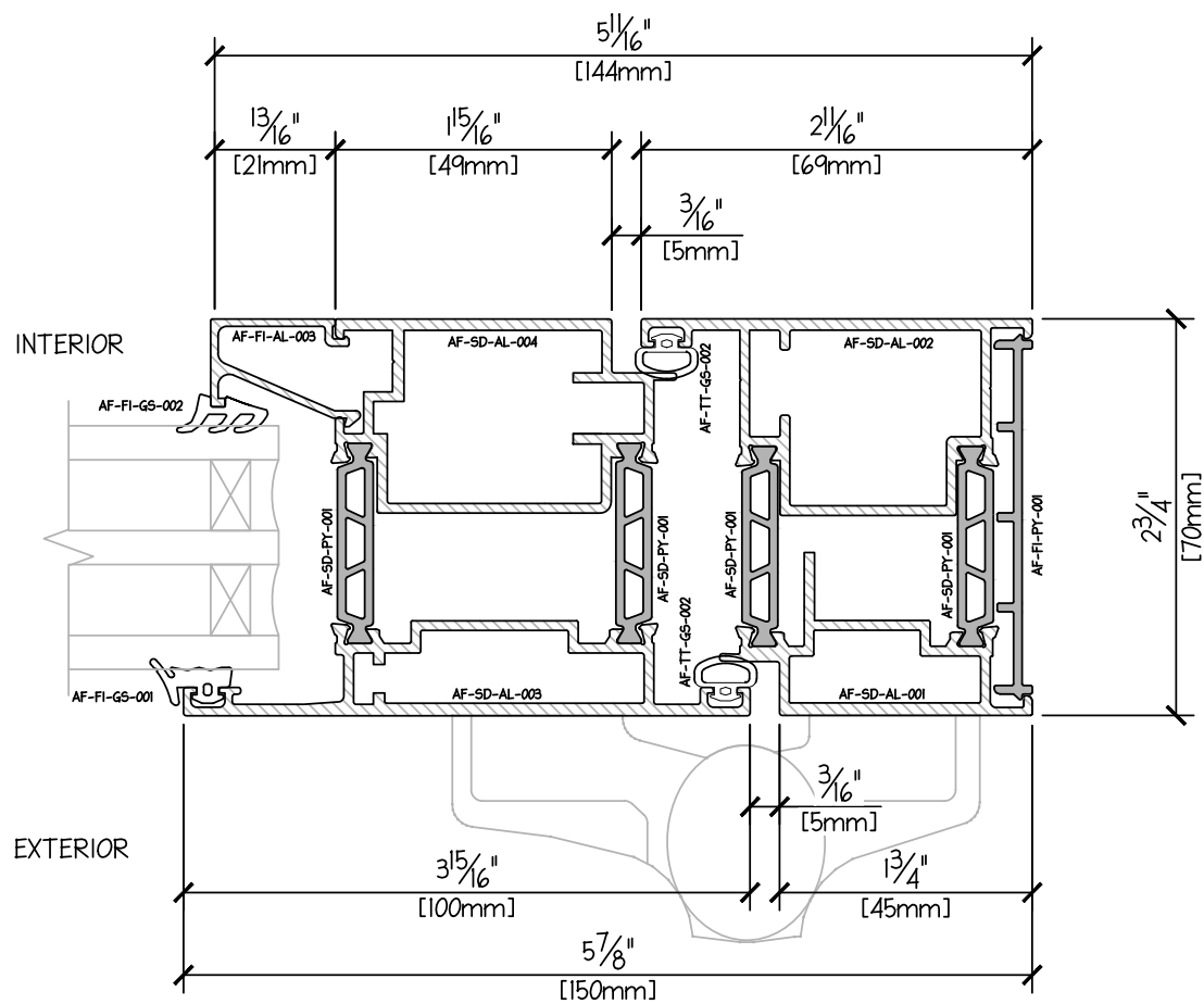
OUTSWING DOOR PROFILE - JAMB - HINGE TRIPLE GLAZE 43mm
