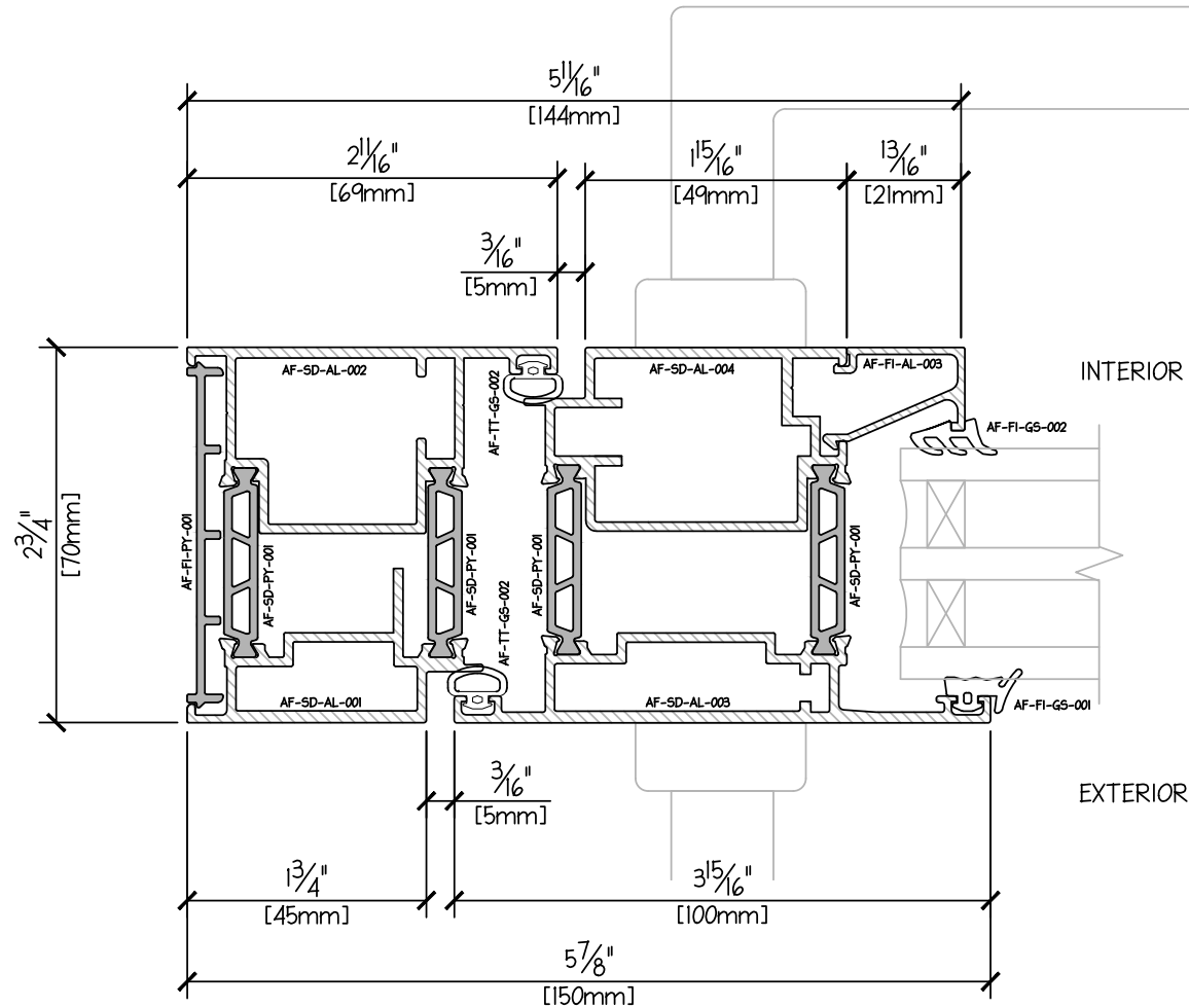
OUTSWING DOOR PROFILE - JAMB - HANDLE TRIPLE GLAZE 43mm
