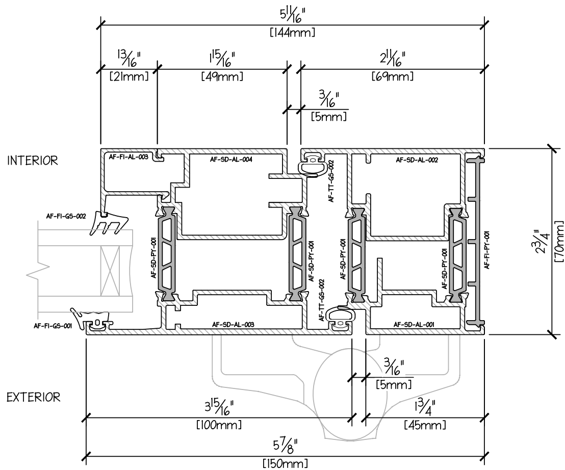
OUTSWING DOOR PROFILE - JAMB - HINGE DUAL GLAZE 31mm
