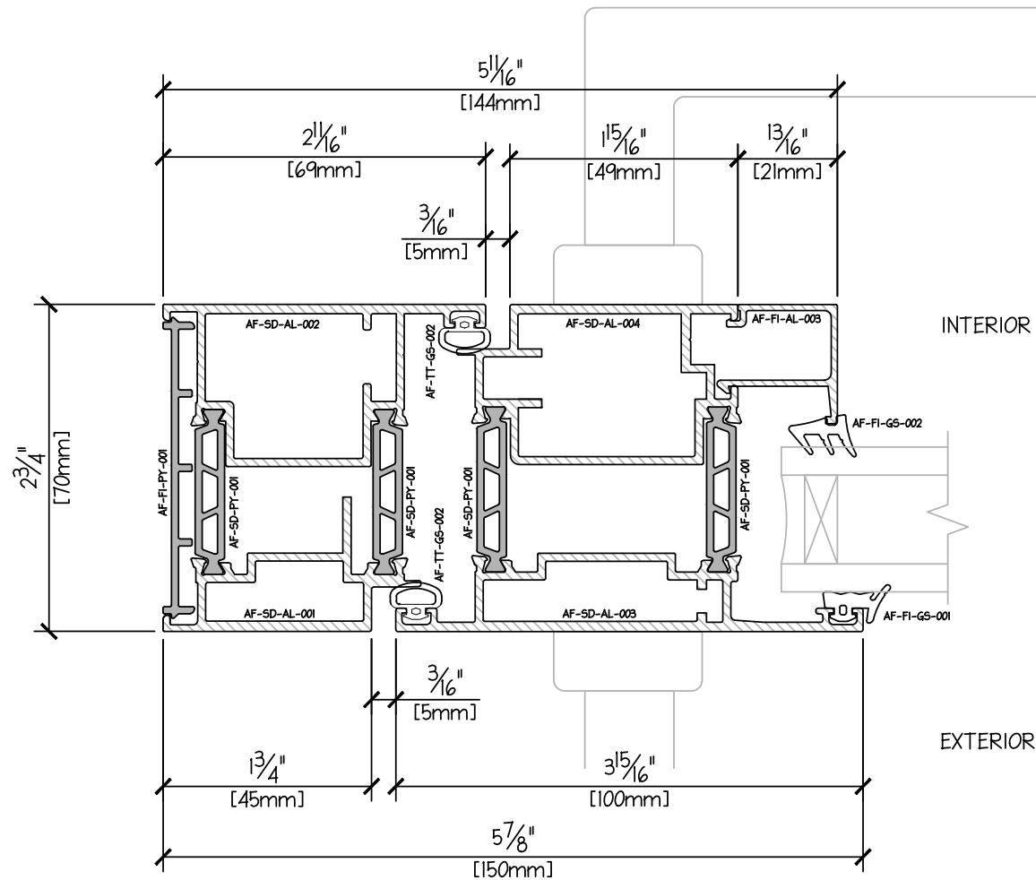
OUTSWING DOOR PROFILE - JAMB - HANDLE DUAL GLAZE 31mm
