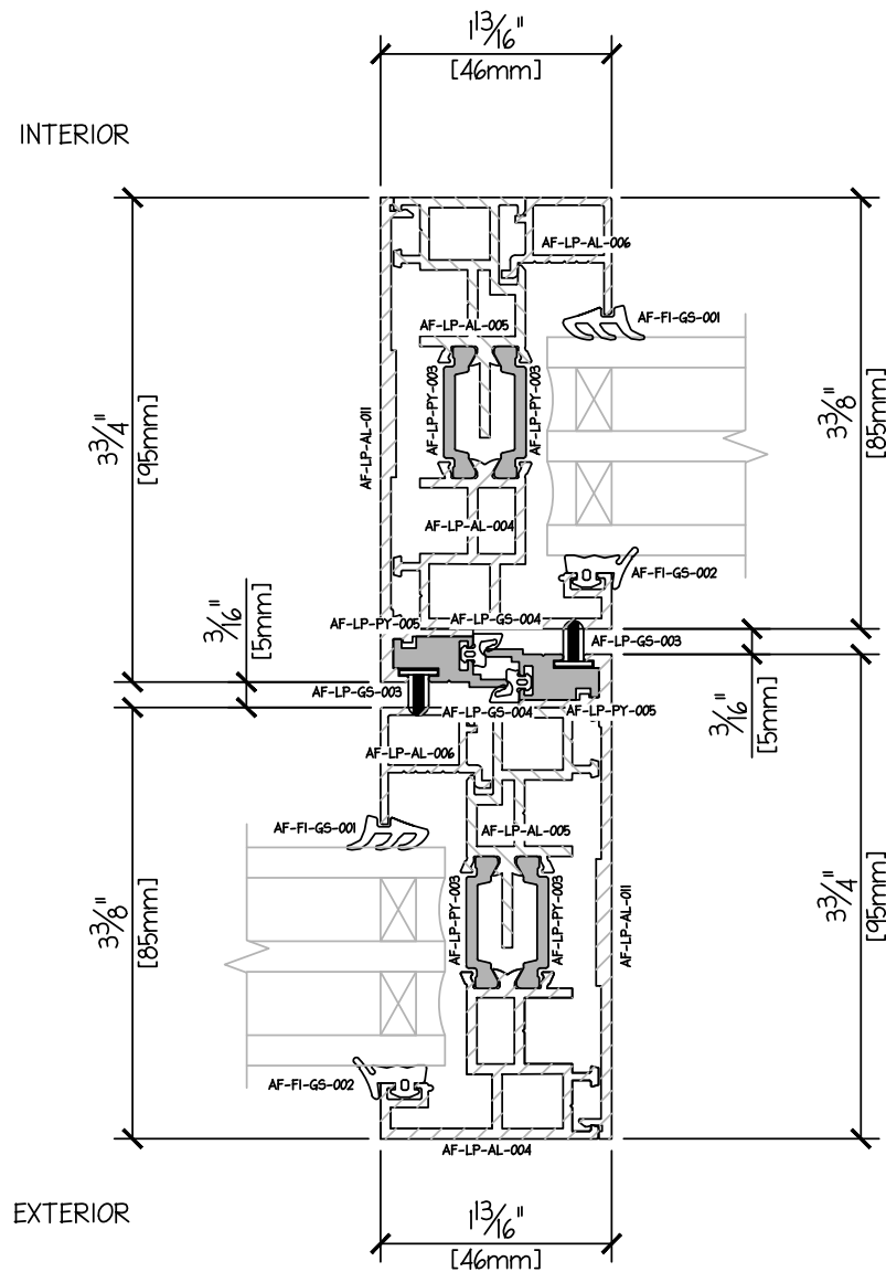
LOW PROFILE SLIDER - INTERLOCK TRIPLE GLAZE 43mm
