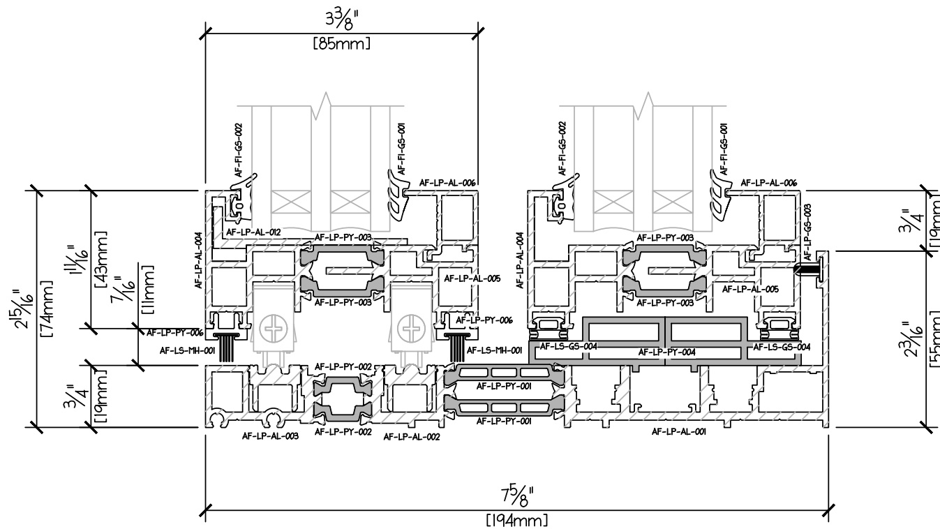
LOW PROFILE SLIDER - SILL @ OPERABLE PANEL TRIPLE GLAZE 43mm
