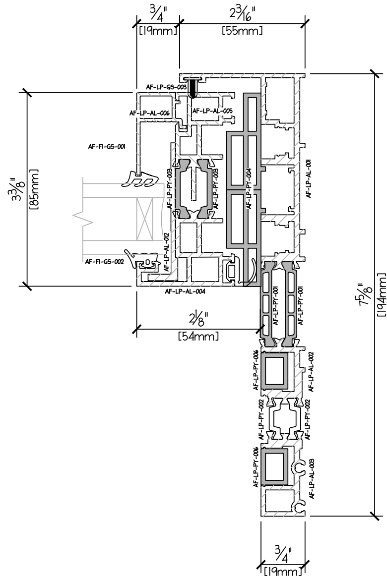
LOW PROFILE SLIDER - JAMB FIXED DUAL GLAZE 32mm
