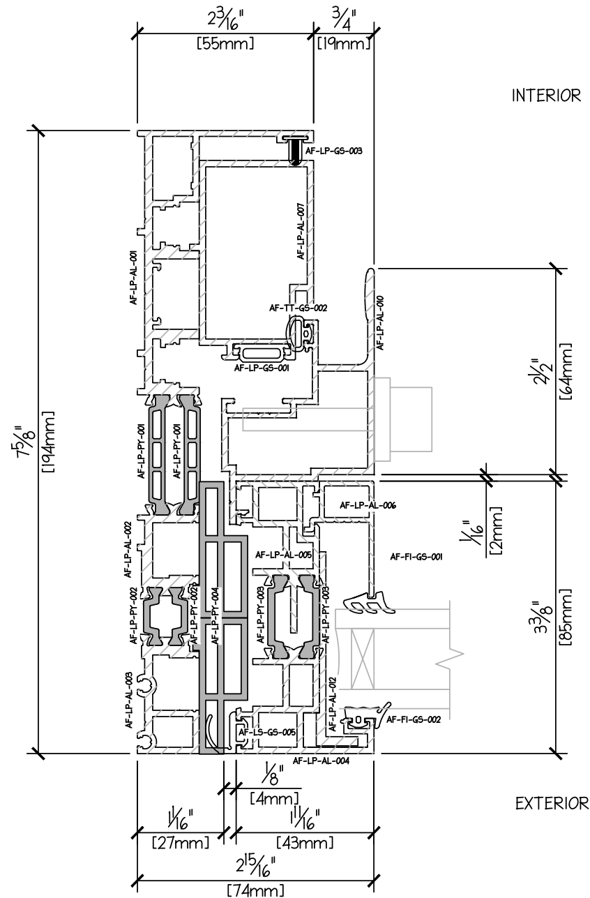
LOW PROFILE SLIDER - JAMB OPERABLE DUAL GLAZE 32mm
