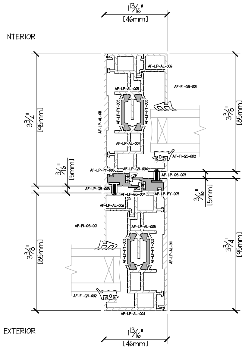
LOW PROFILE SLIDER - INTERLOCK DUAL GLAZE 32mm
