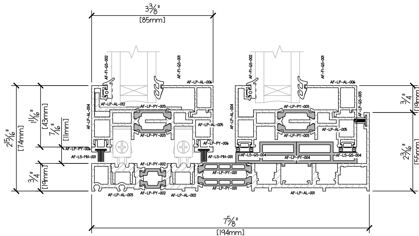
LOW PROFILE SLIDER - SILL @ OPERABLE PANEL DUAL GLAZE 32mm
