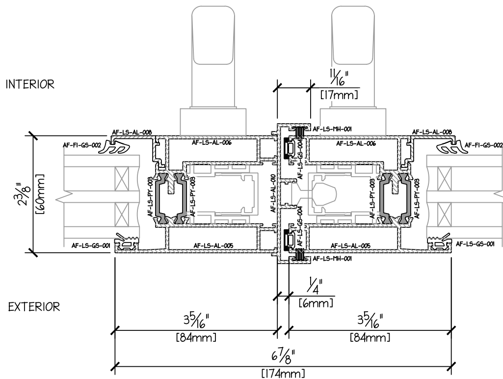
LIFT SLIDE 3 TRACK PROFILE - JAMB - INTERLOCK XX TRIPLE GLAZE 43mm
