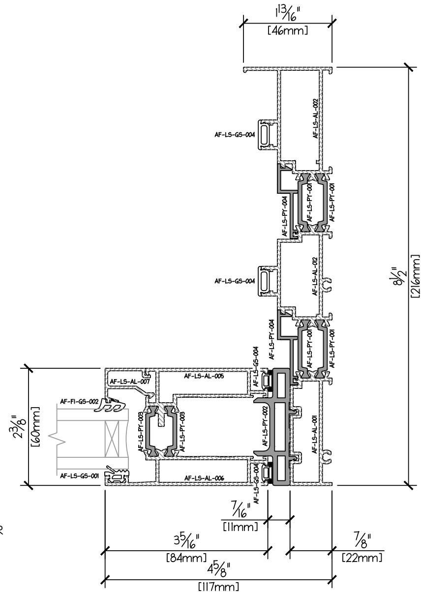
LIFT SLIDE 3 TRACK PROFILE - JAMB - FIXED DUAL GLAZE 31mm
