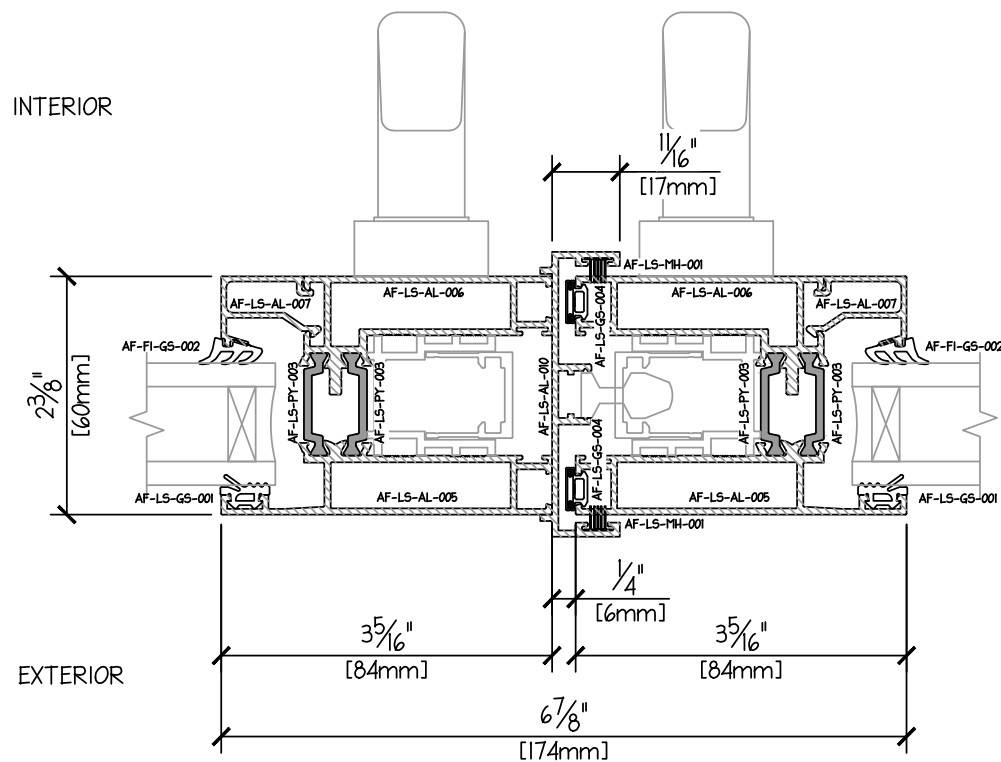
LIFT SLIDE 3 TRACK PROFILE - JAMB - INTERLOCK XX DUAL GLAZE 3mm
