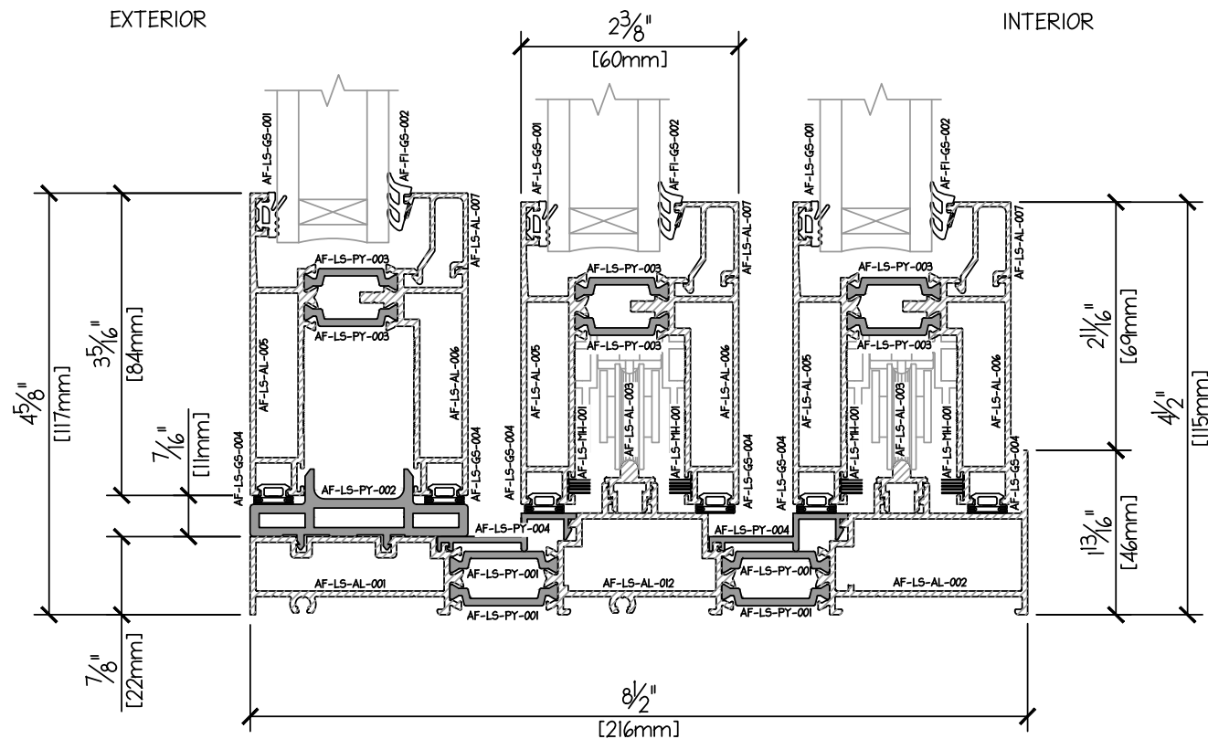
LIFT SLIDE 3 TRACK PROFILE - SILL DUAL GLAZE 31mm
