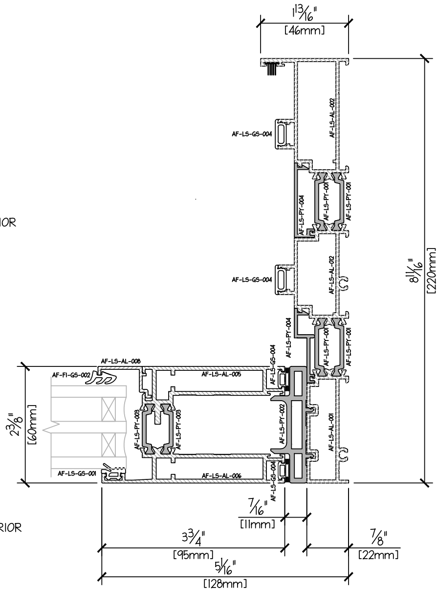
LIFT SLIDE 3 TRACK PROFILE - JAMB - FIXED DUAL GLAZE 31mm
