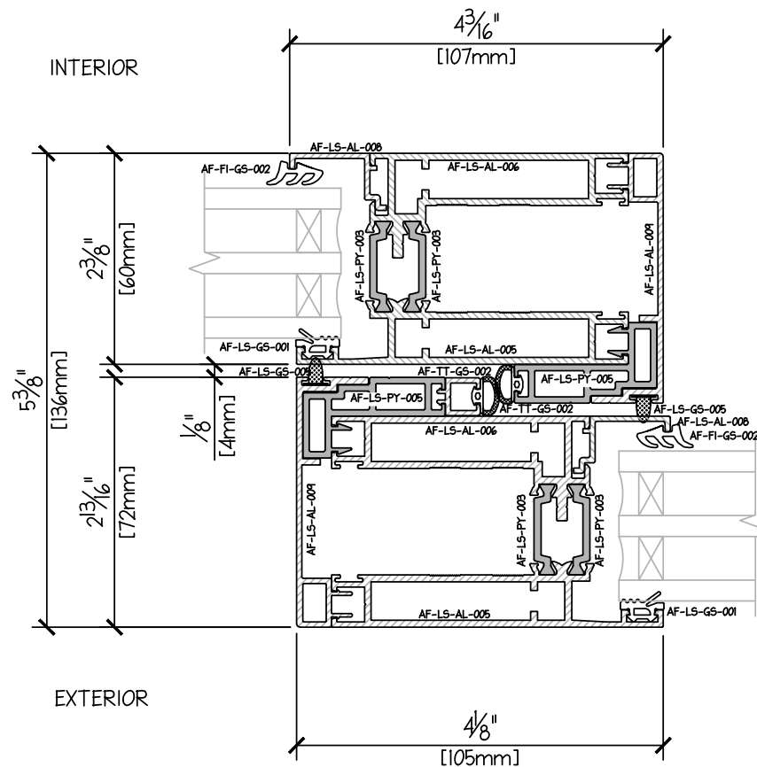
LIFT SLIDE 3 TRACK PROFILE - JAMB - INTERLOCK DUAL GLAZE 31mm
