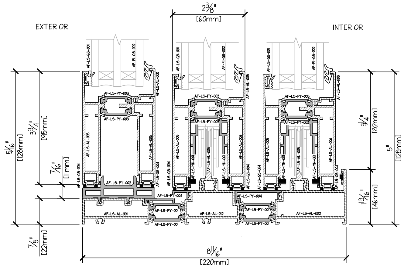
LIFT SLIDE 3 TRACK PROFILE - SILL DUAL GLAZE 31mm
