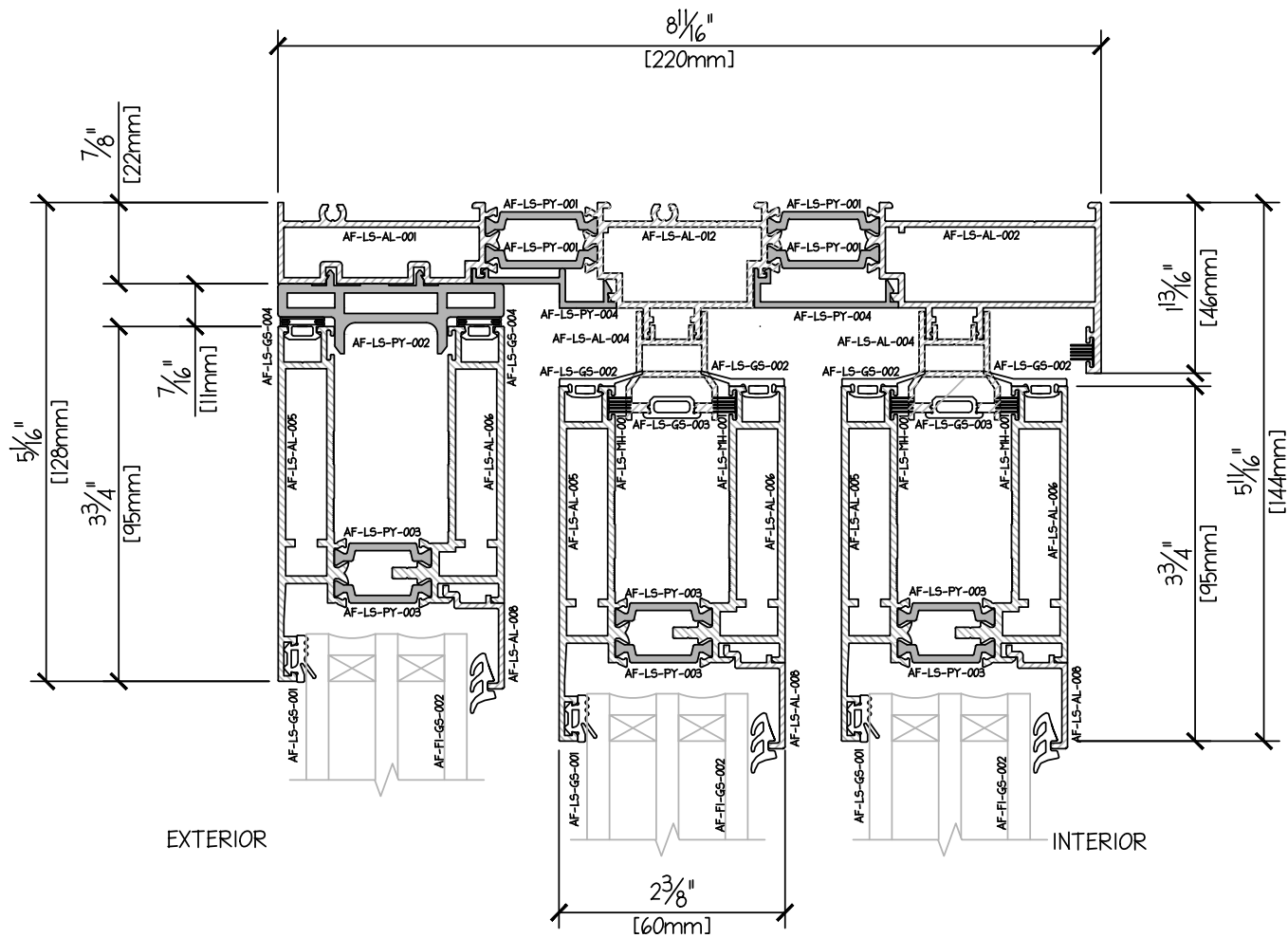
LIFT SLIDE 3 TRACK PROFILE - HEAD DUAL GLAZE 31mm
