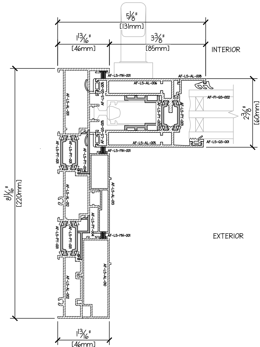
LIFT SLIDE 3 TRACK PROFILE - JAMB - OPERABLE DUAL GLAZE 31mm
