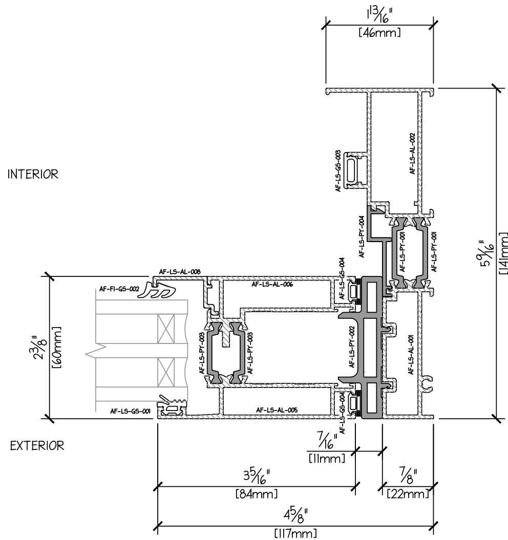
LIFT SLIDE 2 TRACK PROFILE - JAMB - FIXED TRIPLE GLAZE 43mm
