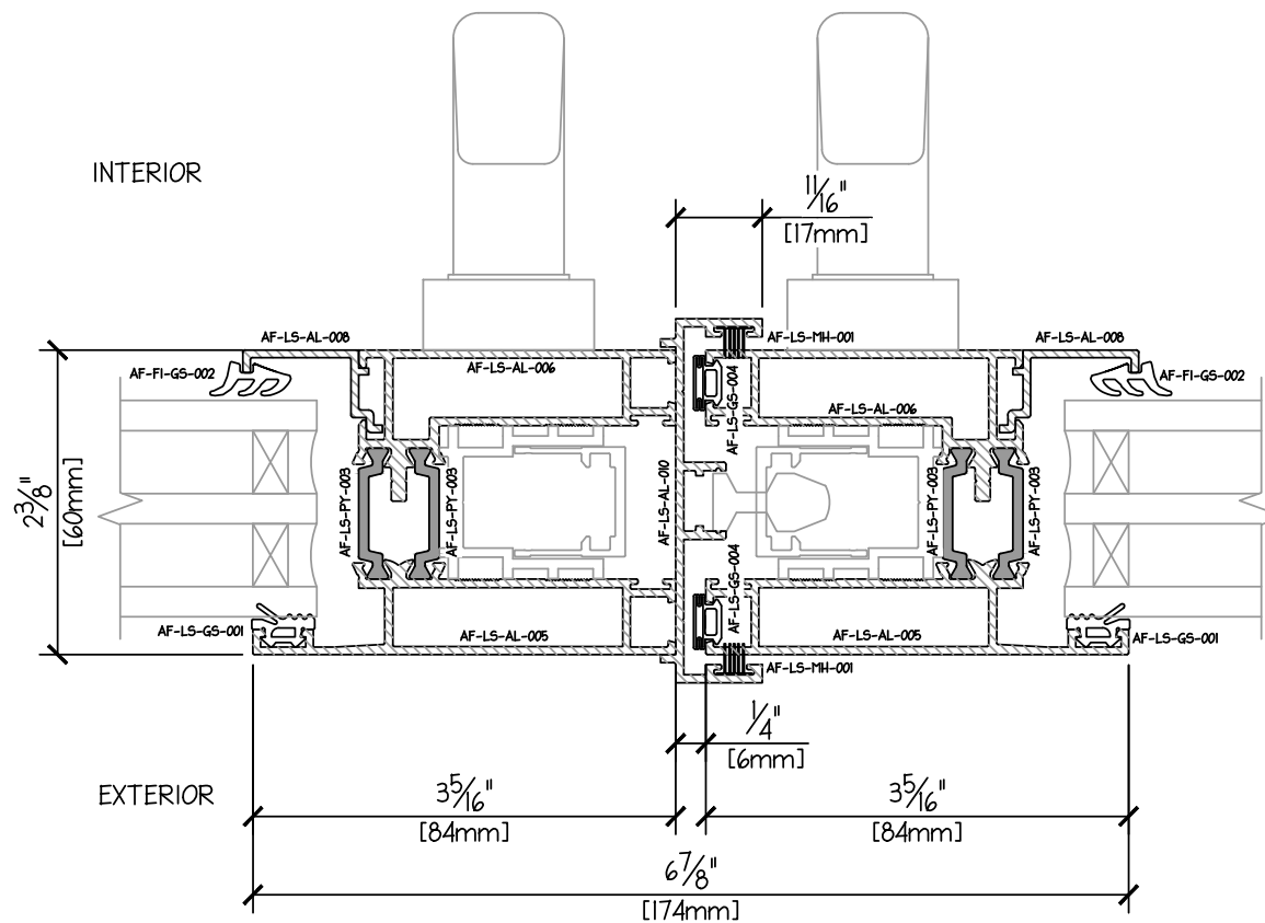
LIFT SLIDE 2 TRACK PROFILE - JAMB - INTERLOCK TRIPLE GLAZE 43mm
