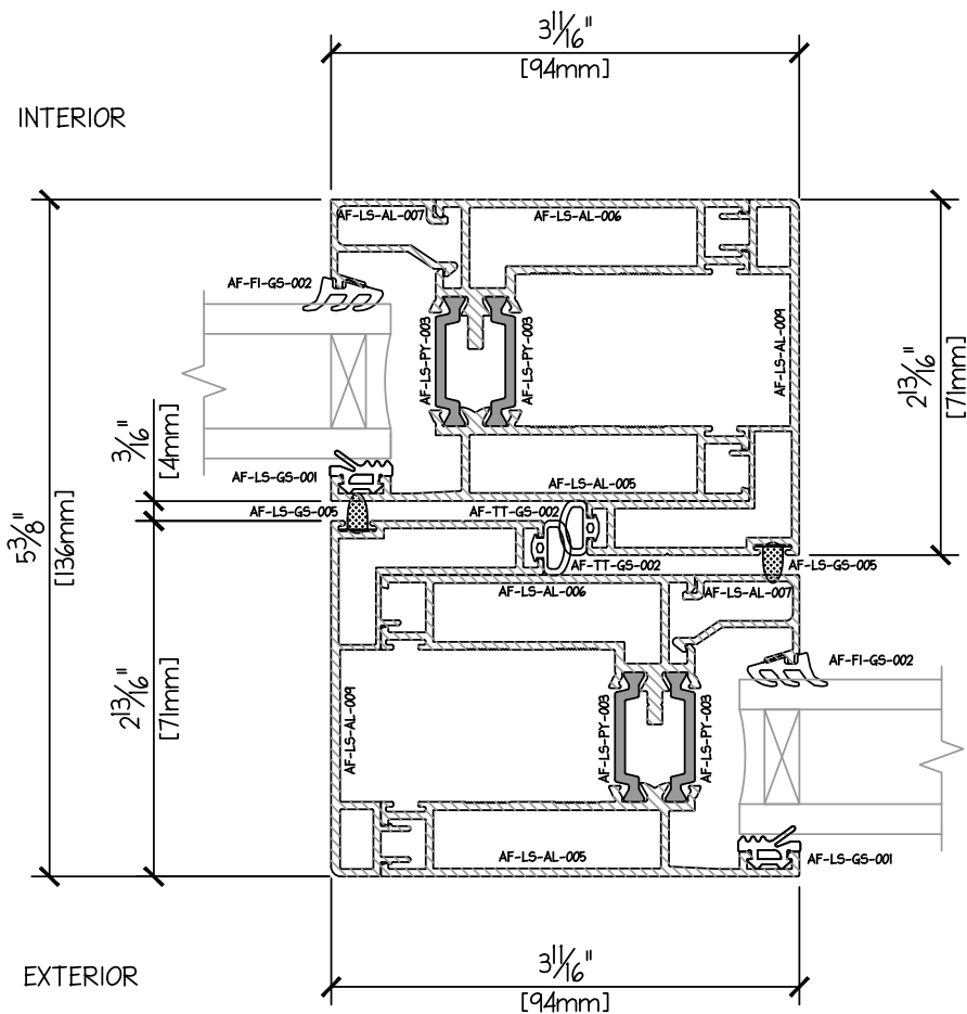
LIFT SLIDE 2 TRACK PROFILE - JAMB - INTERLOCK DUAL GLAZE 31mm
