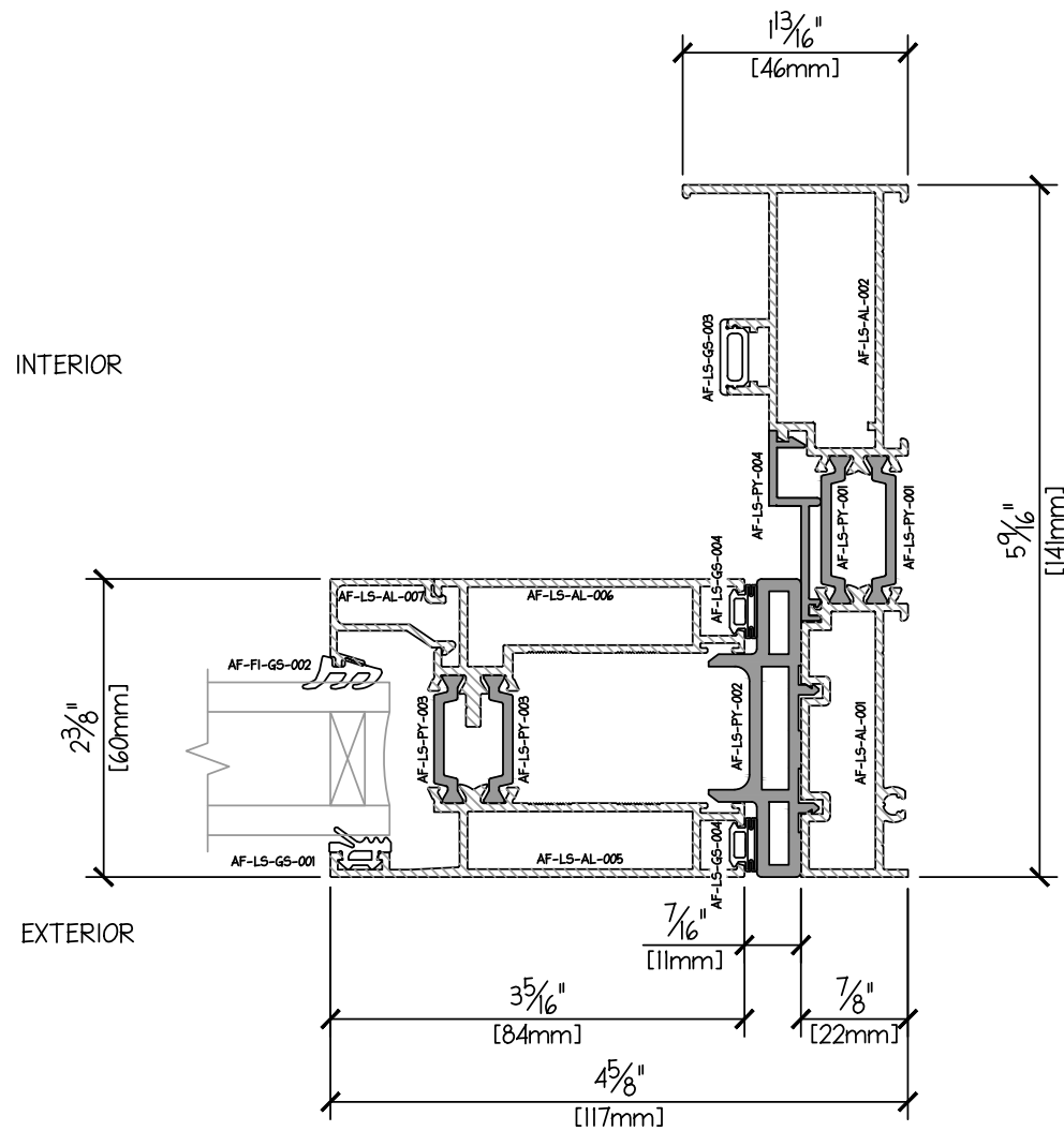
LIFT SLIDE 2 TRACK PROFILE - JAMB - FIXED DUAL GLAZE 31mm
