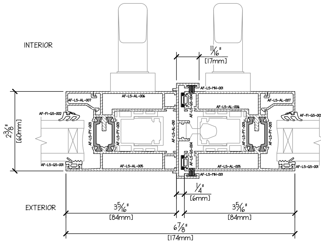
LIFT SLIDE 2 TRACK PROFILE - JAMB - INTERLOCK DUAL GLAZE 31mm
