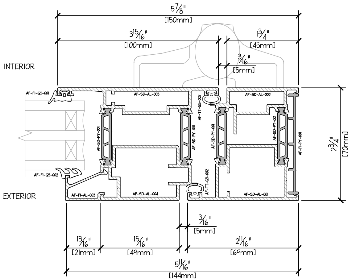
INSWING DOOR PROFILE - JAMB - HINGE TIPLE GLAZE 43mm
