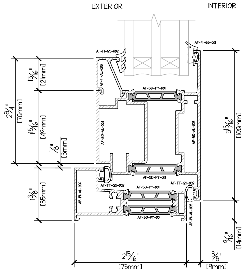
INSWING DOOR PROFILE - SILL TRIPLE GLAZE 43mm
