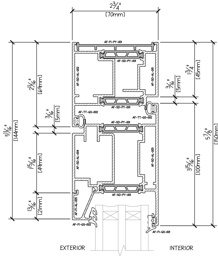
INSWING DOOR PROFILE - HEAD TRIPLE GLAZE 43mm
