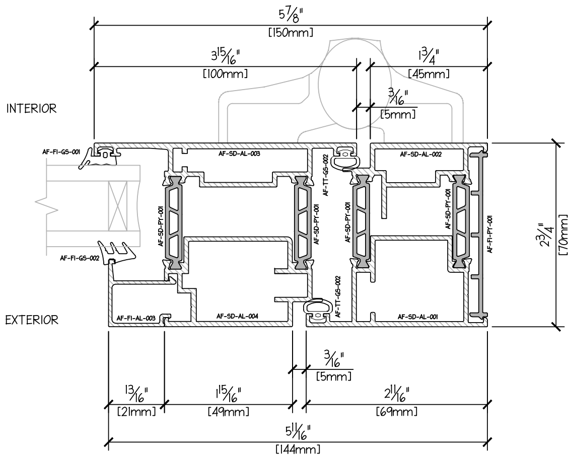
INSWING DOOR PROFILE - JAMB - HINGE DUAL GLAZE 31mm
