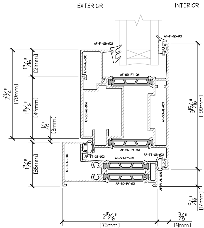
INSWING DOOR PROFILE - SILL DUAL GLAZE 31mm
