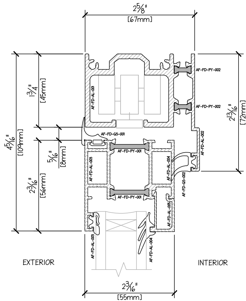
OUTSWING FOLDING DOOR PROFILE - HEAD DUAL GLAZE 31mm
