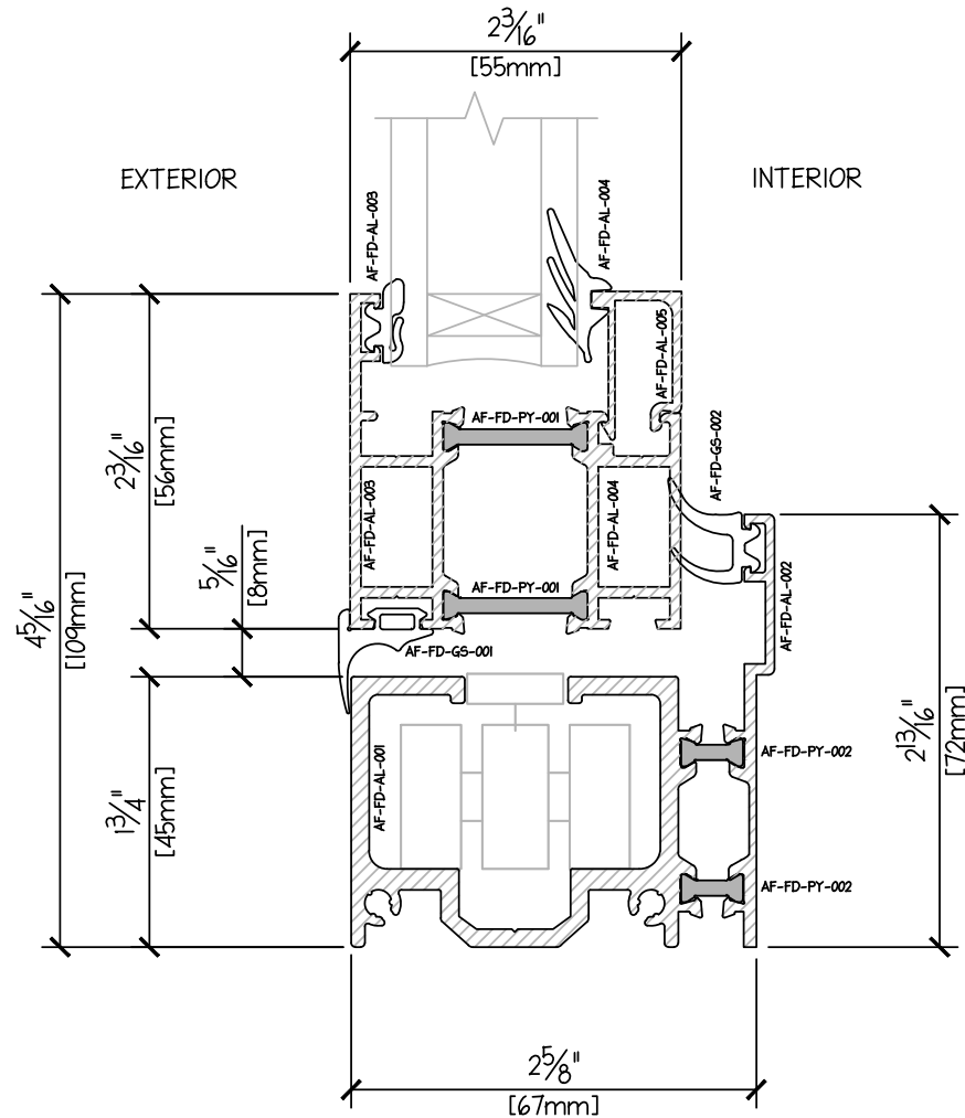
OUTSWING FOLDING DOOR PROFILE - SILL HIGH DUAL GLAZE 31mm
