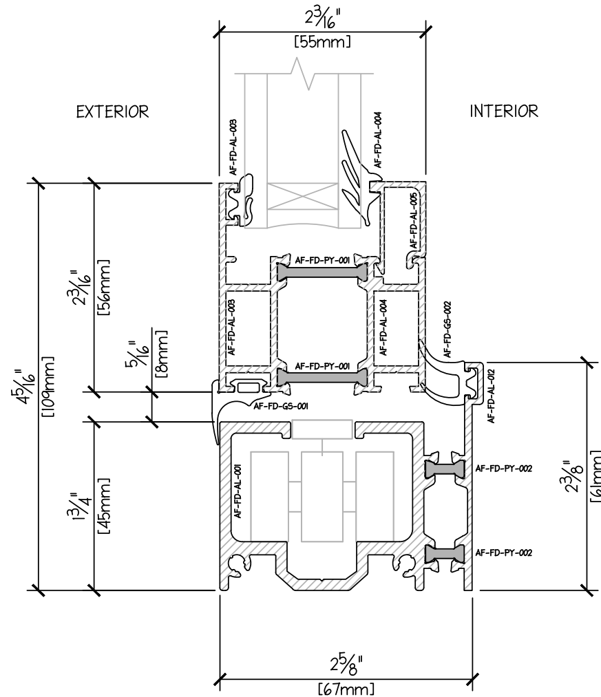
OUTSWING FOLDING DOOR PROFILE - SILL LOW DUAL GLAZE 31mm
