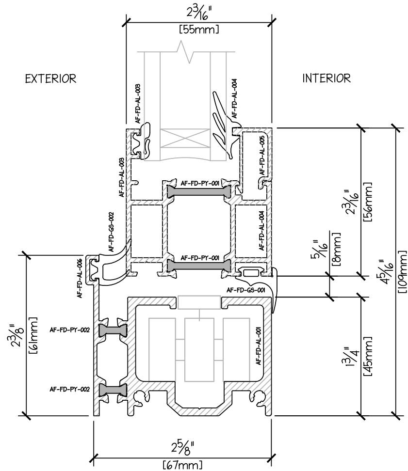
INSWING FOLDING DOOR PROFILE - SILL LOW DUAL GLAZE 31mm
