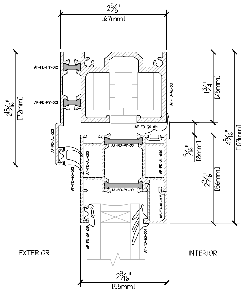
INSWING FOLDING DOOR PROFILE - HEAD DUAL GLAZE 31mm
