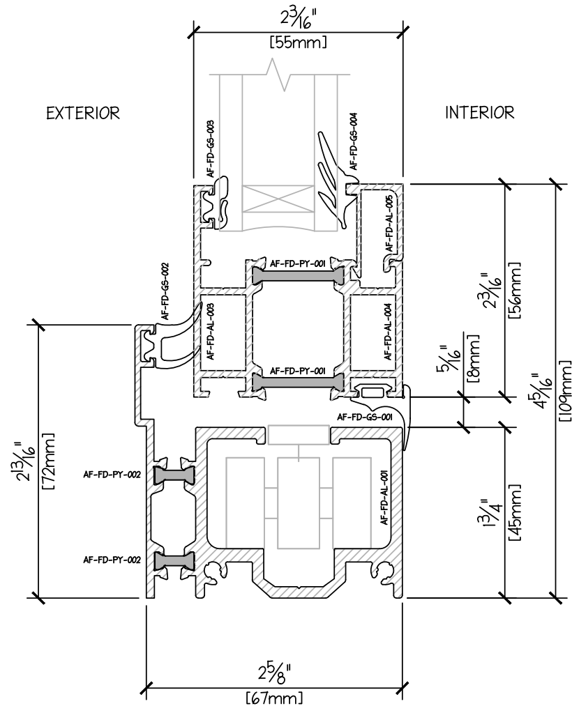
INSWING FOLDING DOOR PROFILE - SILL HIGH DUAL GLAZE 31mm
