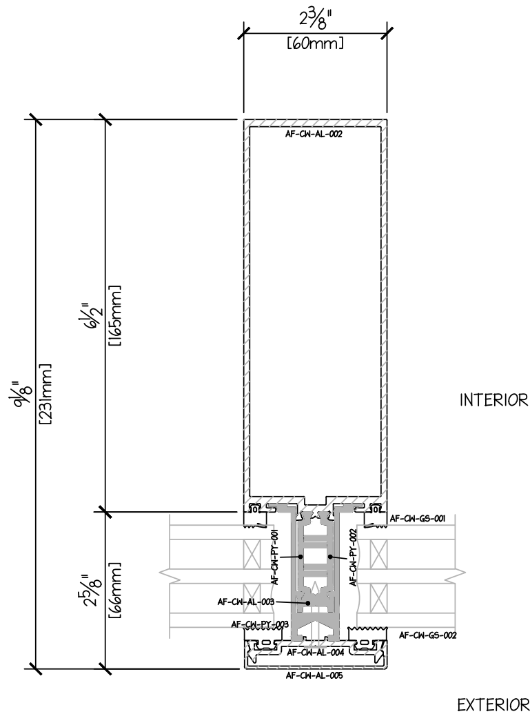
CURTAIN WALL 6 1/2" - VERTICAL MULLION TRIPLE GLAZE 43mm
