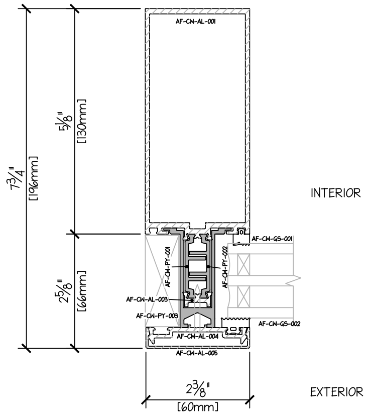
CURTAIN WALL 5 1/8" - JAMB TRIPLE GLAZE 43mm
