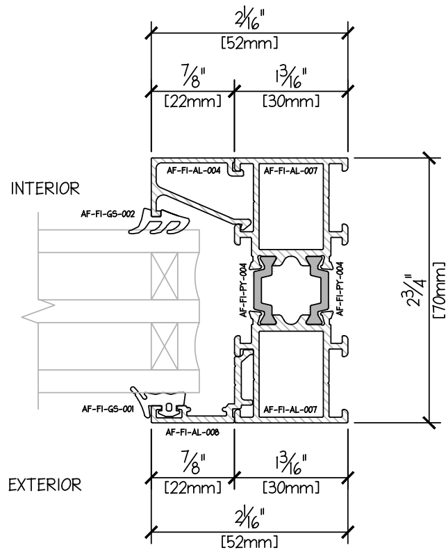
CASEMENT-FIXED PROFILE - JAMB TRIPLE GLAZE 43mm
