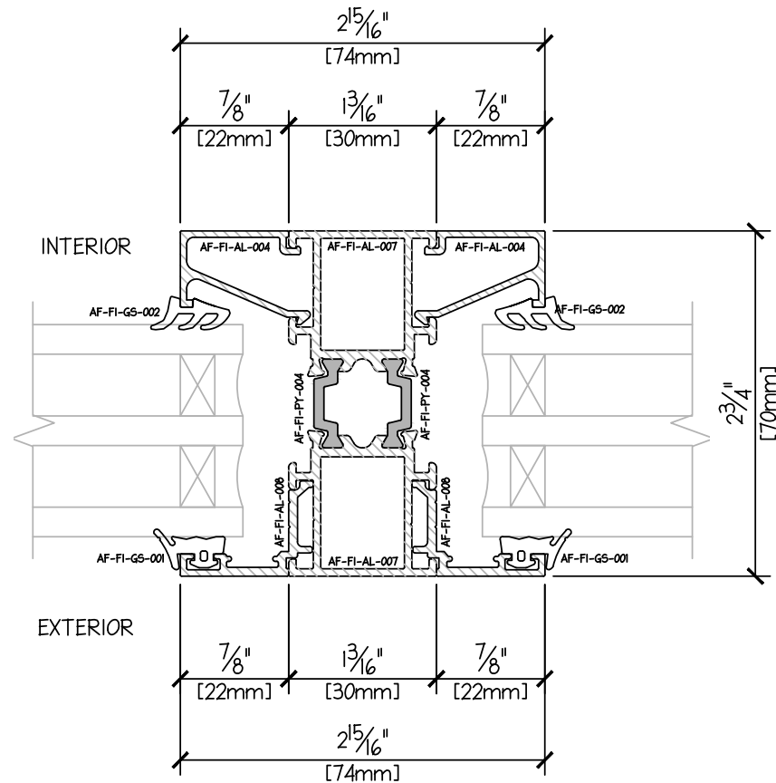
CASEMENT-FIXED PROFILE - VERTICAL MULLION TRIPLE GLAZE 43mm
