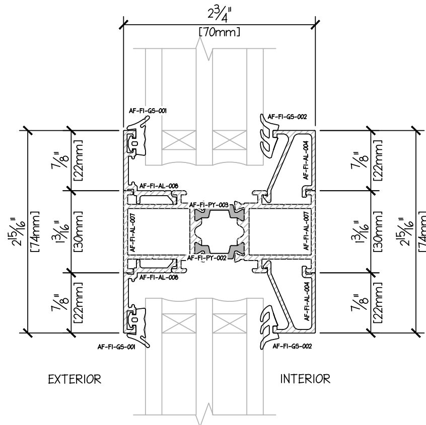
CASEMENT-FIXED PROFILE - HORIZONTAL MULLION TRIPLE GLAZE 43mm
