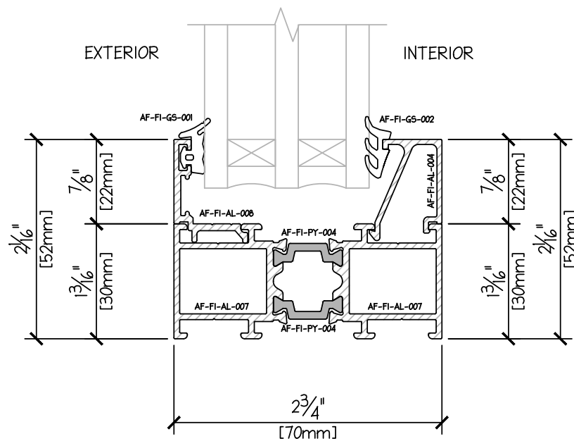
CASEMENT-FIXED PROFILE - SILL TRIPLE GLAZE 43mm
