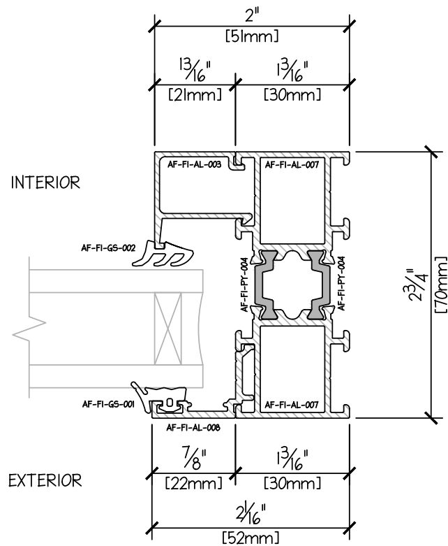
CASEMENT-FIXED PROFILE - JAMB DUAL GLAZE 31mm
