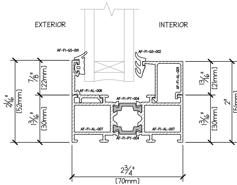
CASEMENT-FIXED PROFILE - SILL DUAL GLAZE 31mm
