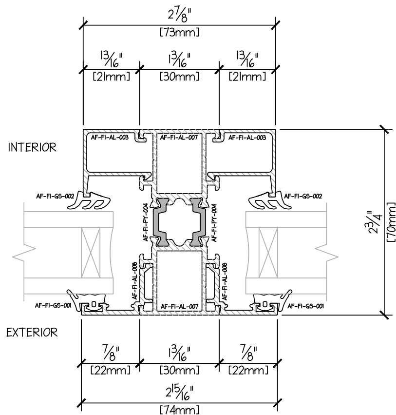
CASEMENT-FIXED PROFILE - VERTICAL MULLION DUAL GLAZE 31mm
