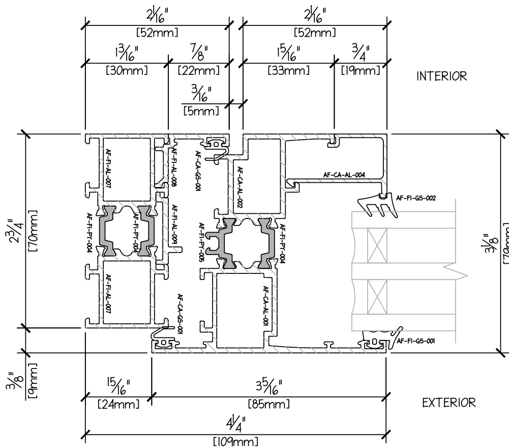
AWNING PROFILE - JAMB TRIPLE GLAZE 43mm
