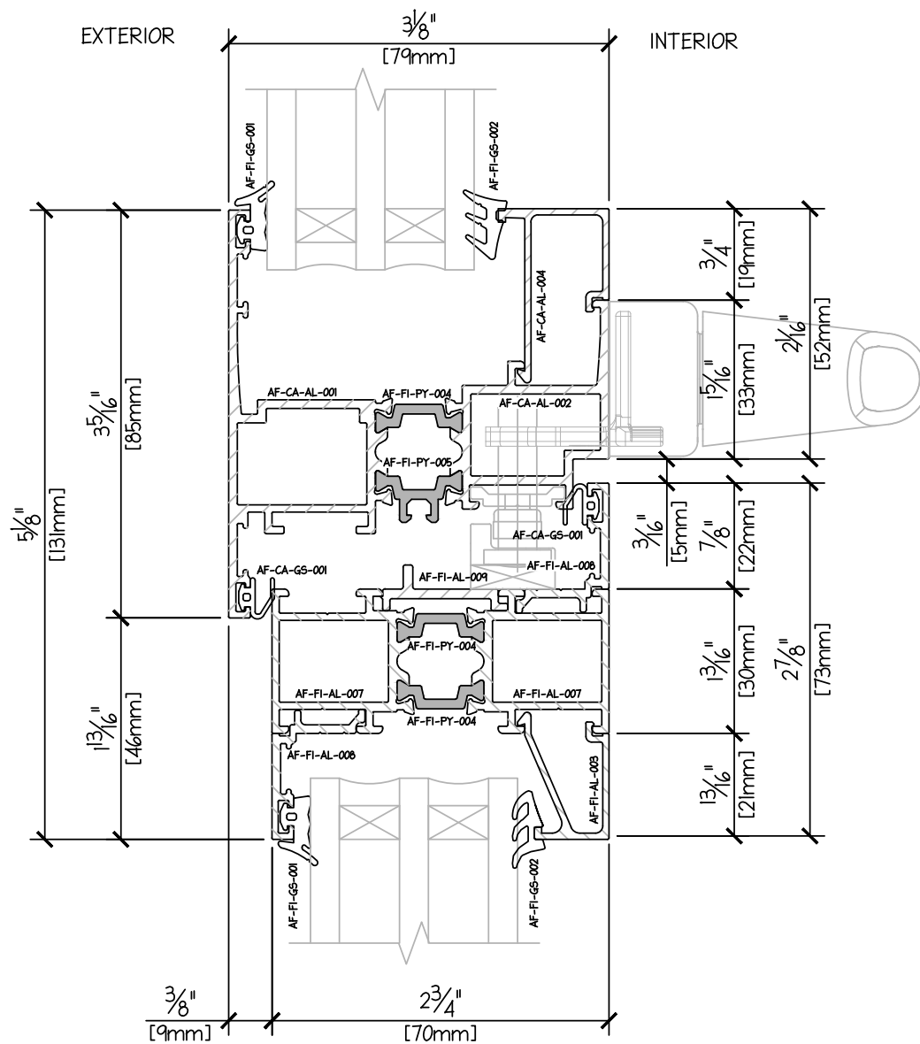
AWNING PROFILE - MULLION - OP/OP - VERTICAL TRIPLE GLAZE 43mm
