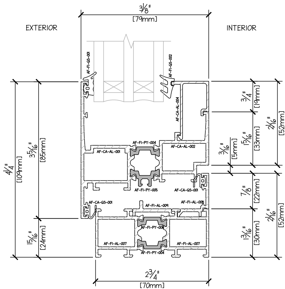
AWNING PROFILE - SILL TRIPLE GLAZE 43mm
