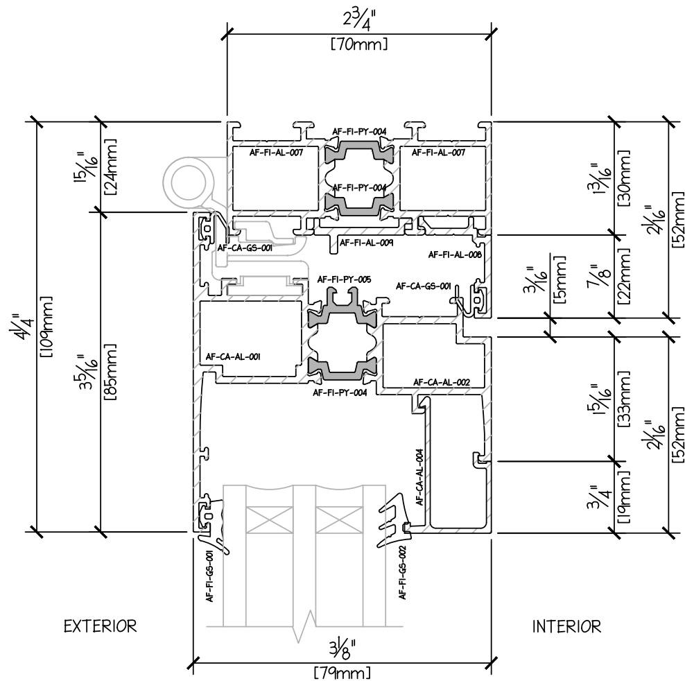
AWNING PROFILE - HEAD TRIPLE GLAZE 43mm
