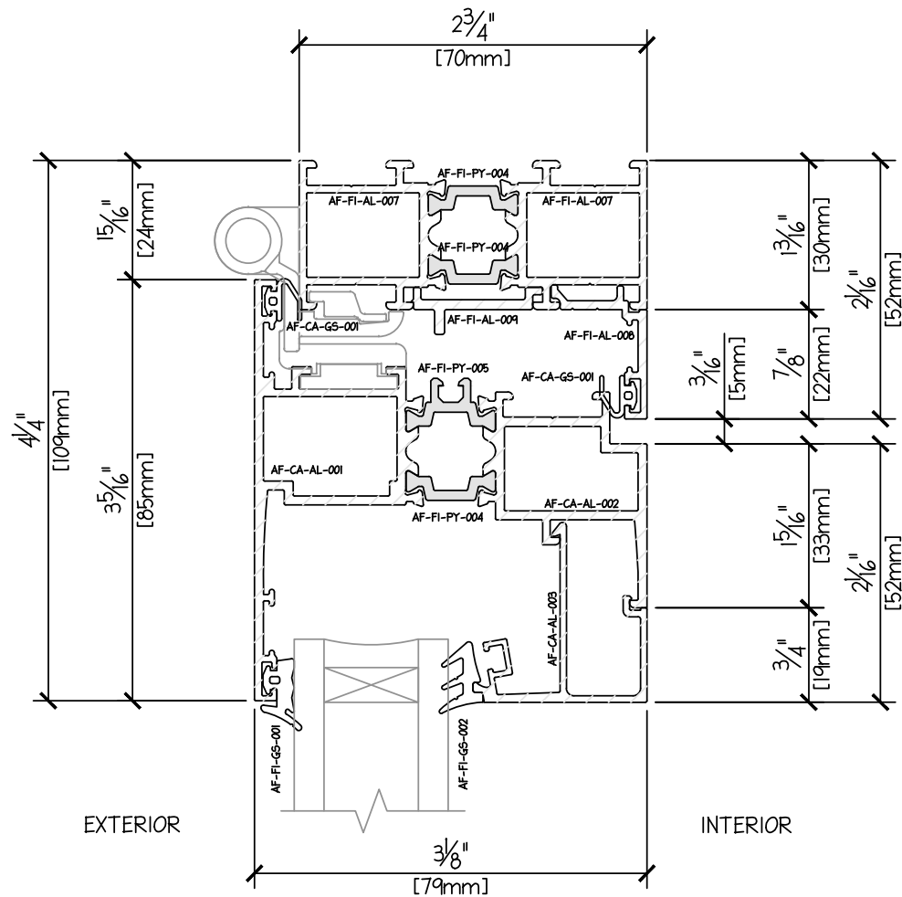
AWNING PROFILE - HEAD DUAL GLAZE 31mm
