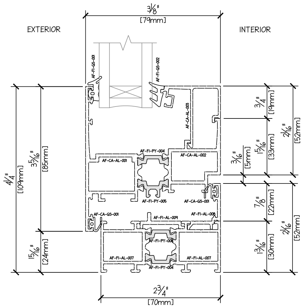
AWNING PROFILE - SILL DUAL GLAZE 31mm
