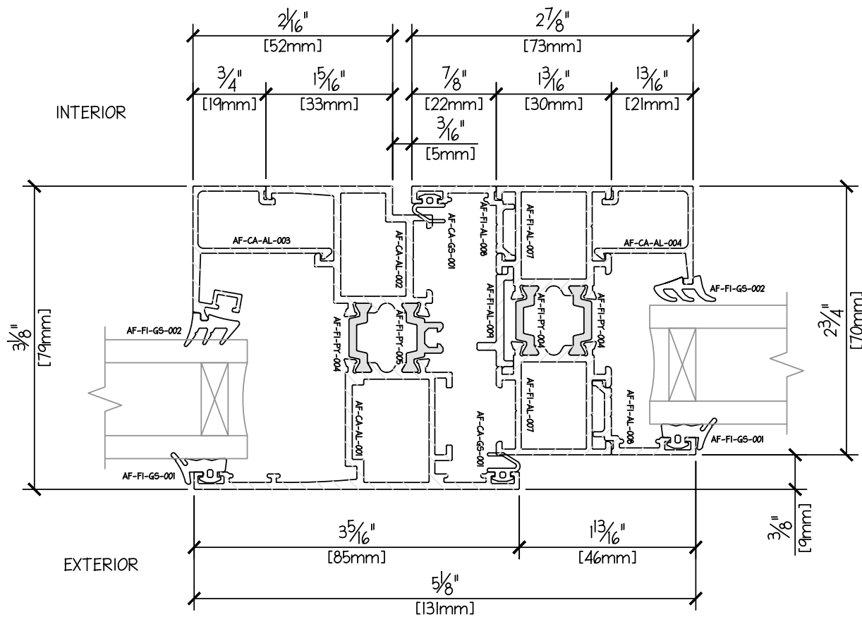
AWNING PROFILE - MULLION - OP/FIX - HORIZONTAL DUAL GLAZE 31mm
