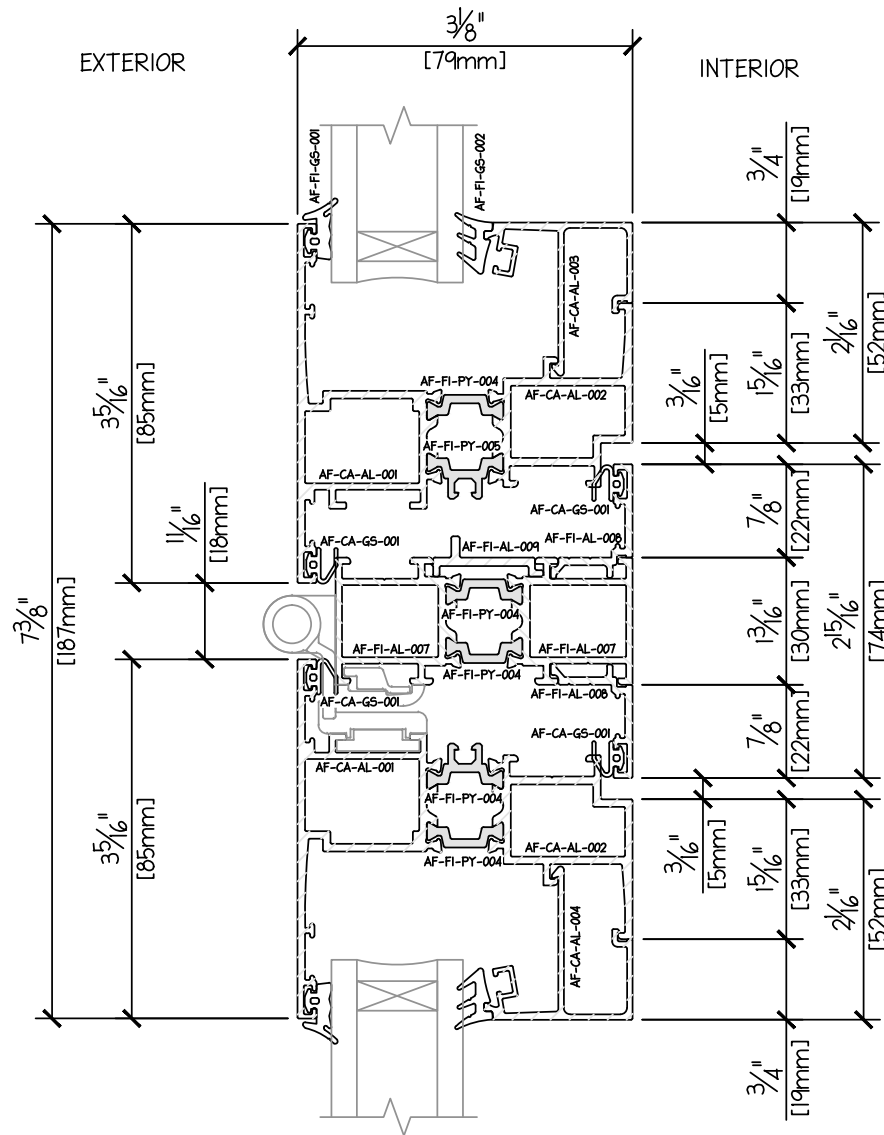
AWNING PROFILE - MULLION - OP/OP - VERTICAL DUAL GLAZE 31mm
